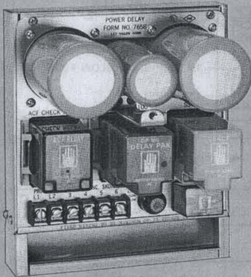
FORM 7658 POWER DELAY MODULE With Cover Removed
