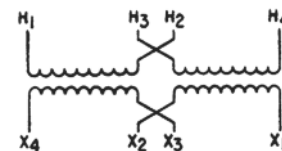
Wiring Diagram for Low Voltage Loads
