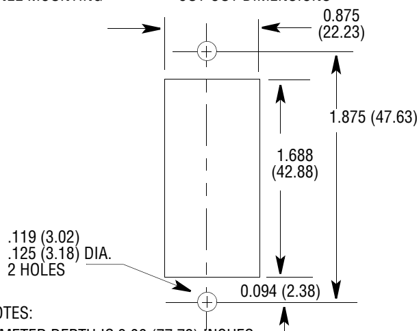
PANEL MOUNTING
